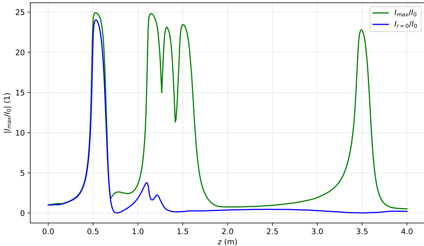
I_{max}(x = 0, y = 0, z)/I_0 , P_{in}=4.4P_{cr} , noisy input, artificial time
